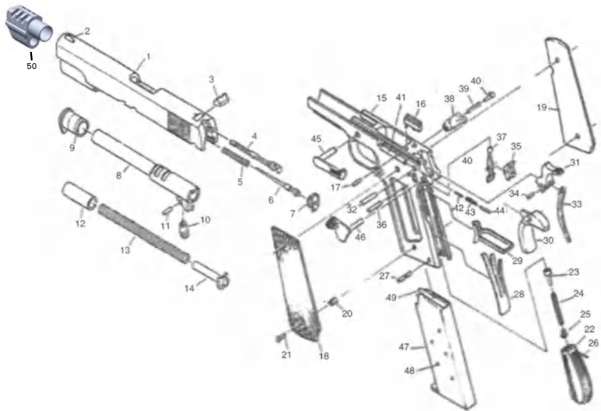
FIGURE 12-BALIKLI 1911 SPORT PARTS ILLUSTRATION
